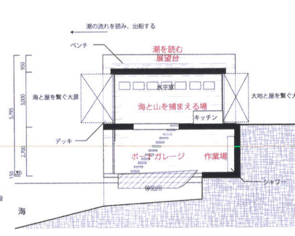
SECTION(1:150)
